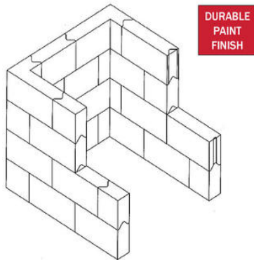
042-434 3 Wall Lead Brick Cave for 042-433
